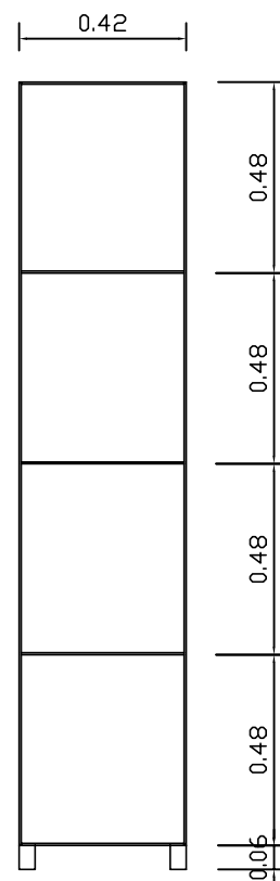
VISTA FRONTAL
