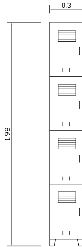
VISTA FRONTAL
