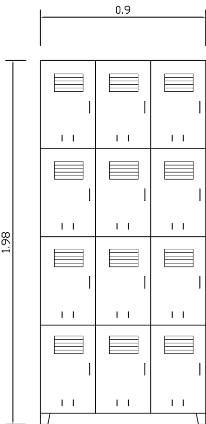
VISTA FRONTAL
